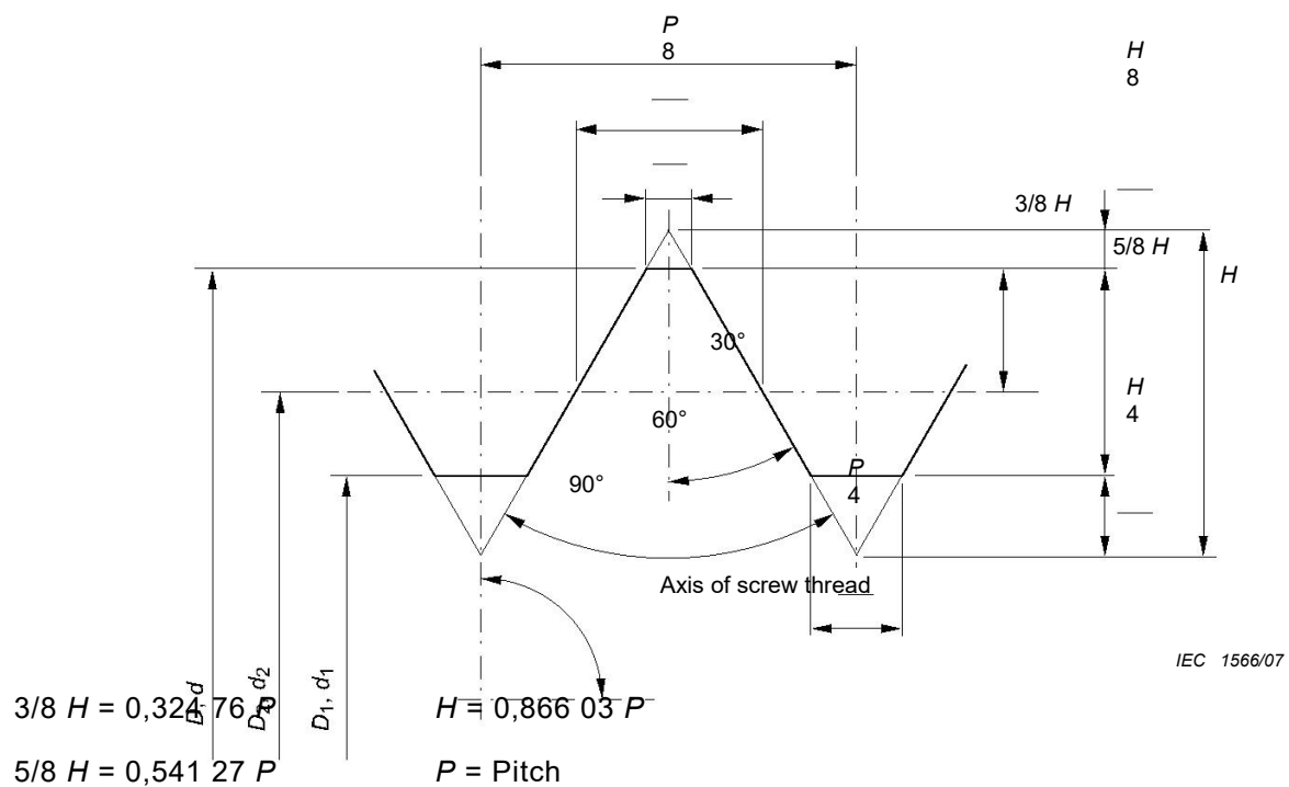
Figure 1 – Basic profile of screw threads
